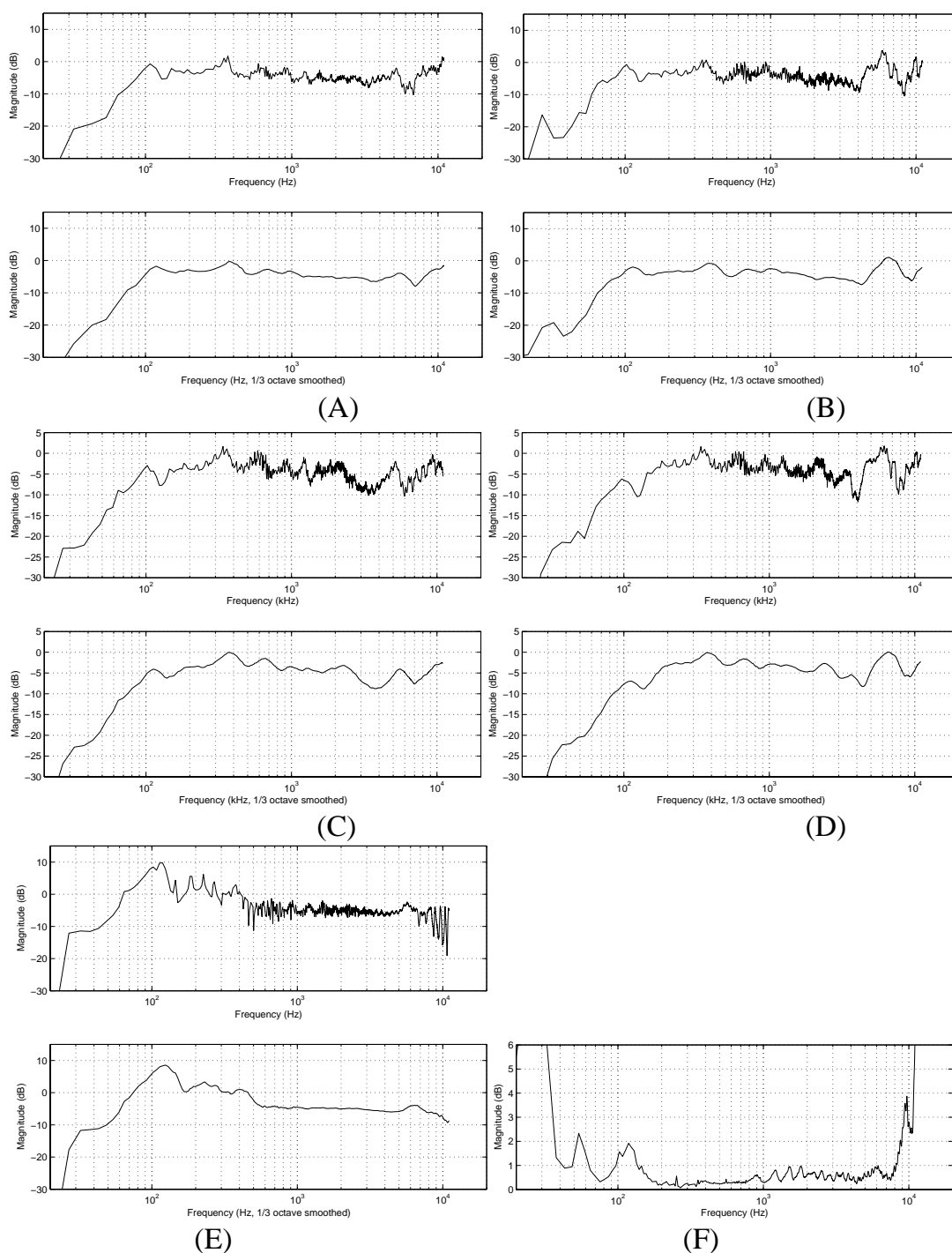
Figure 18. Frequency responses (MLSSA) of the tubeophone sound system. In each plot, the top panel shows raw 4096 point FFT with 22050 Hz sampling rate and the bottom panel shows 1/3 octave smoothed version of it (near auditory frequency resolution). Measurements in summer 2004: Original loudspeaker element using tube 1 (A), with tube 2 (B), Replacement loudspeaker installed in 2002 spring, tube 1 (C) tube 2 (D). Original design phase measurement (E). Standard deviation with four subsequent placement of different ear tips (F).
