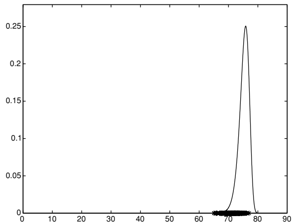
Figure 4. The minimum angles between the estimated components in the whitened space, using the quasi-orthogonalization approach on image data. Asterisks: The minimum angles between the estimated image basis vectors. Solid line: The distribution this quantity would have, if the vectors were drawn randomly.
