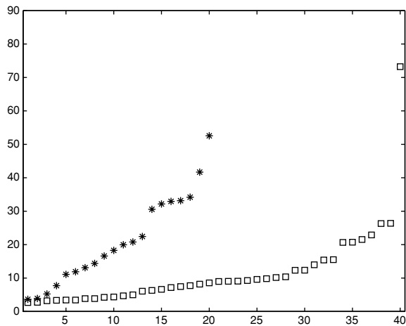
Figure 12. The angles between the real basis vectors and the matched estimates, for simulated data using the gaussianization procedure. Squares: Laplacian distributed sources estimated with the present algorithm. Asterisks: For comparison, estimation of complete basis using ordinary FastICA, in deflation mode.
