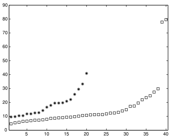
Figure 2. The angles between the real and matched components, using the quasi-orthogonalization approach. Squares: Laplacian distributed sources estimated with the present algorithm. Asterisks: For comparison, estimation of complete basis using FastICA, in symmetric mode.
