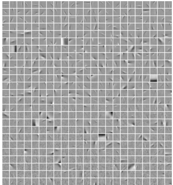
Figure 13. The image basis vectors obtained with the method using gaussianization. The order in which the vectors were obtained was left upper-hand corner to right lower-hand corner, scanning row by row. The upper half of the plot thus shows what one would obtain if one only estimated a 2 time overcomplete basis. The whole set of vectors gives a 4 times overcomplete basis.
