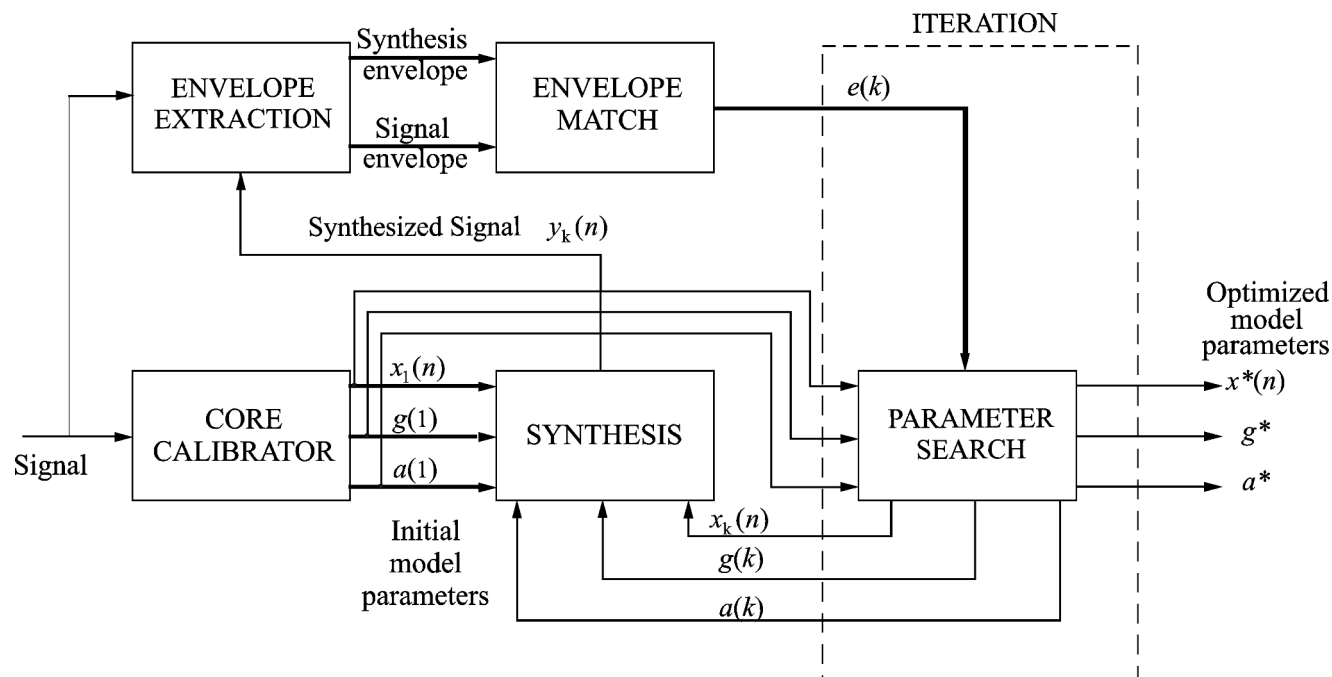
Figure 3. An extended iterative parameter extraction scheme that matches the overall decay of the analyzed and synthesized sounds, after Erkut et al. (2000).
