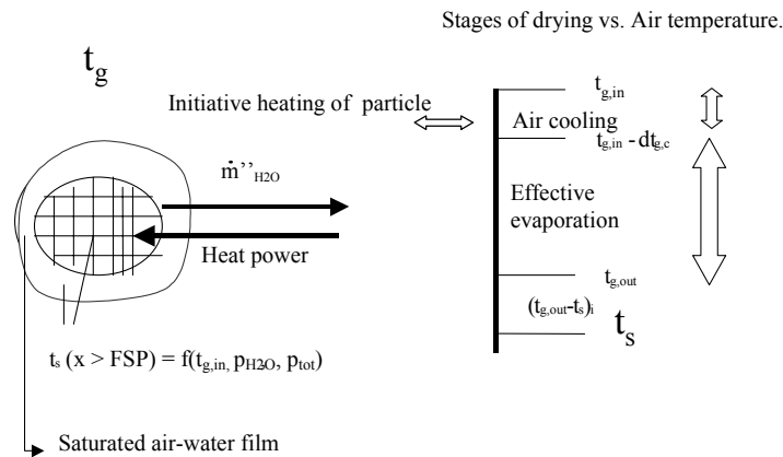
Figure 3. Particle drying.
