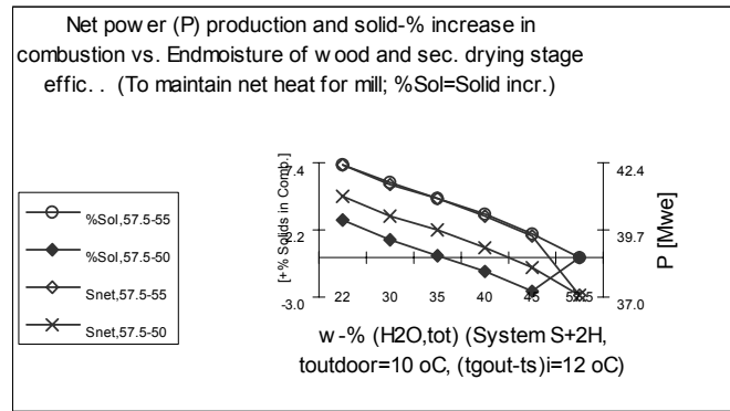
Figure 5. Solid increase (%) in combustion to maintain initial net heat for mill.
