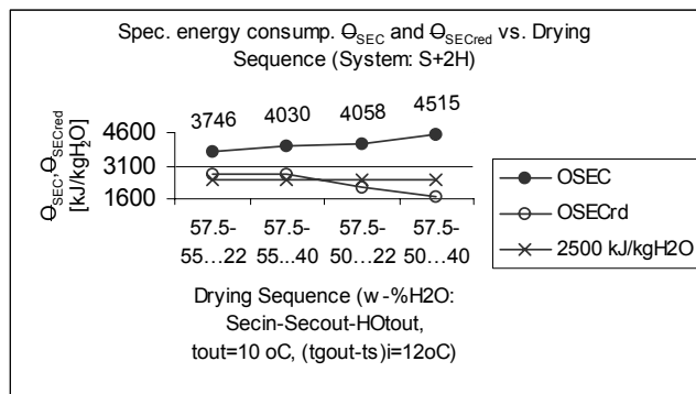
Figure 7. Specific ( \Phi_{SEC} ) and reduced ( \Phi_{SECred} ) specific energy consumptions of MSDS vs. Drying sequence in MSDS (S+2H)
