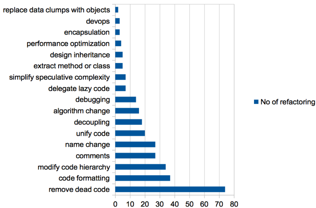
Figure 6: Number of refactorings per driver
