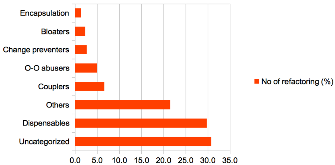
Figure 7: Number of refactorings per code smell taxonomy
