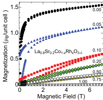
FIG. 3. (Color online) Magnetization-field curves for \text{La}_{0.8}\text{Sr}_{0.2}\text{Co}_{1-x}\text{Rh}_x\text{O}_{3-\delta} at 5 K.
