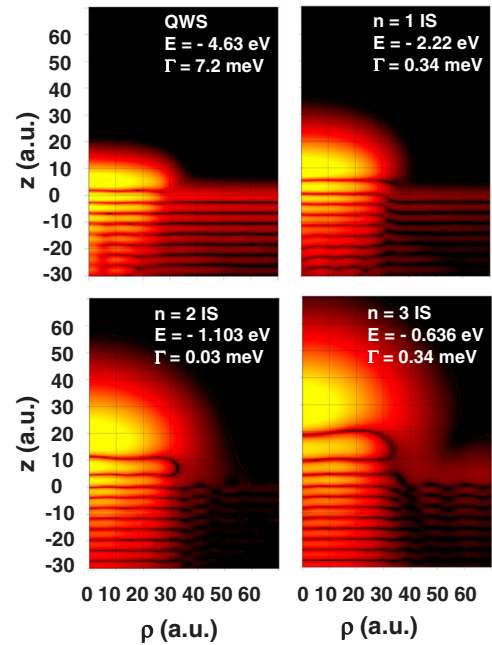
FIG. 2. (Color online) Interpolated images of the electron density of the (m=0, j=0) quasistationary island-localized states for the 61 Na atom island on the Cu(111) surface. The states are labeled according to their parent continua. The natural logarithm of the density is shown in cylindrical coordinates. z=0 corresponds to the position of the image plane of the Cu(111) surface, and inside the metal z is negative. The vacuum edge of the Na island is at z=5.0 a.u. The electron density decreases from 1 to 0.001 (arbitrary units) when going from bright to dark. The energies E [with respect to the vacuum level of Cu(111)] and the widths \Gamma of the states are given in the insets.
