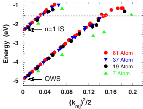
FIG. 1. (Color online) Energy of various (m, j) states for Na atom nanoislands on Cu(111). The energy is referred to the Cu(111) vacuum level. Results are shown as a function of the quantized wave vectors of the corresponding “particle in a box states” (see text for definition). Different symbols represent the states corresponding to the Na islands of different size, as shown in the inset. The dashed gray line shows the position of the vacuum level for the 1 ML Na/Cu(111) system.
