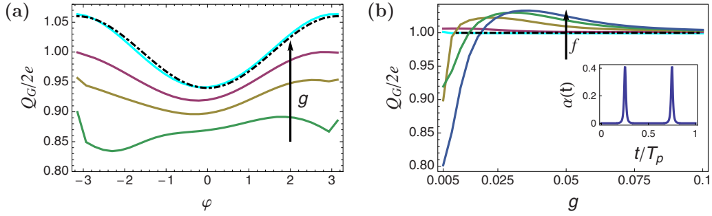
FIG. 2. (Color online) Pumped charge per cycle in a Cooper-pair sluice for zero-temperature environment (a) as a function of phase \varphi with coupling constant g=C_E/C_\Sigma=0.01, 0.0125, 0.015, and 0.1 from bottom to top for f=1/T_p=75 MHz, and (b) as function of coupling g with \varphi=\pi/2 and at frequencies f=10, 25, 50, 65, and 75 MHz from bottom to top in the region in which the arrow is plotted. In the numerical simulations, the parameters are J_i^M/E_C=0.1, J_i^m/J_i^M=0.03 (with i=L,R ), \delta n_g^M=-\delta n_g^m=0.3, E_C/k_B=1 K [ E_C/(2\pi\hbar)=21 GHz], R=300 k \Omega , environment temperature T=0, S(\omega_0)=2\hbar\omega_0R, S(-\omega_0)=0, and S(0)=2k_B T_0 R with T_0=0.1 K. In inset we show the time evolution of the adiabatic parameter \alpha(t) for f=75 MHz.
