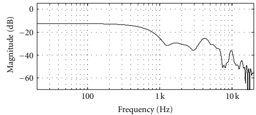
FIGURE 10: Isolation curve of an ARA headset.
