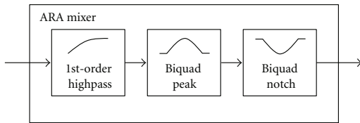
FIGURE 5: Equalization block diagram of the ARA mixer [4].
