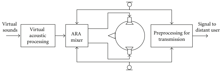
FIGURE 1: Block diagram of an ARA system.
