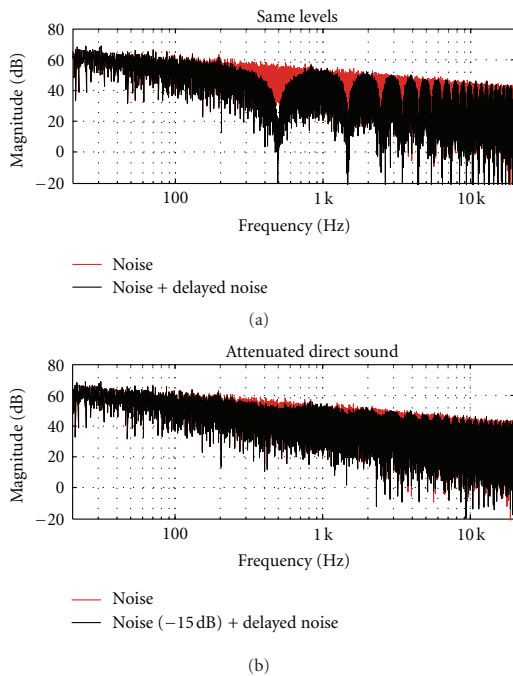
FIGURE 17: Comb filtering effect with the delay of 1 ms. The red curve represent the spectrum of pink noise and the black curve represents the spectrum of pink noise which is added to the delayed version of itself. (a) illustrates the comb filtering effect, when the added signals have the same energy, whereas (b) illustrates the effect when the passive attenuation of the ARA headset is considered.
