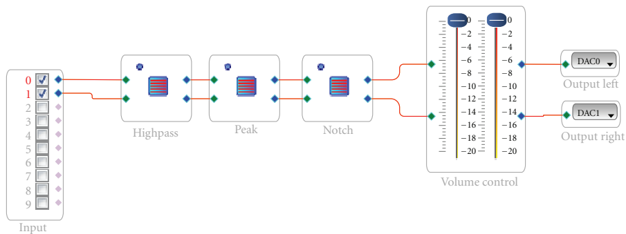
FIGURE 14: SigmaStudio implementation of the ARA equalizer.
