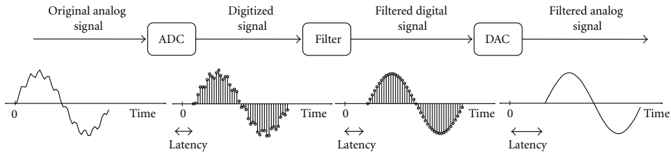
FIGURE 9: Basic functionality and latency of a digital filter.
