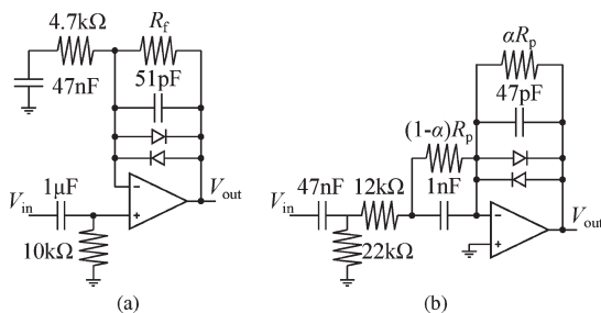
Fig. 4. Distortion circuits used in the simulations. (a) Noninverting distortion [5]. (b) Inverting distortion [10].
