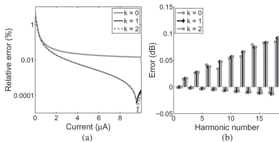
Fig. 3. Evaluation of the diode model for k = 0, 1 , and 2 iterations for the Lambert W function approximation with a sinusoidal input. (a) Voltage approximation error as a function of the diode current. (b) Error for approximating individual harmonics.
